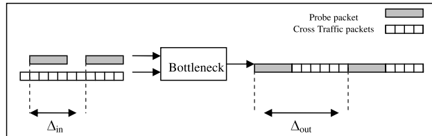
Figure 2: The Probe Gap Model (PGM) for estimating available bandwidth.
