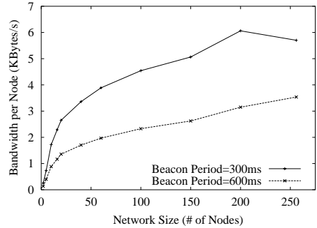
Figure 19. Cost of Monitoring. Here we show bandwidth used for fault-detection as a function of overlay network size. Individual curves represent different monitoring periods, and bandwidth is measured in kilobytes per second per node.
